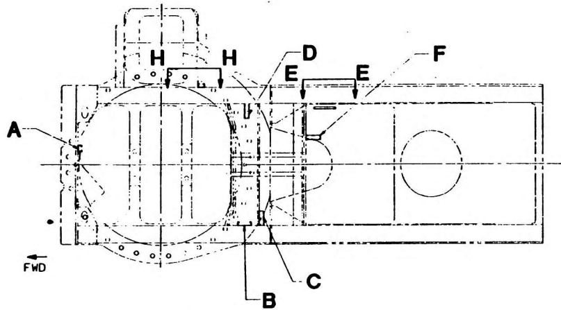
PLAN VIEW OF TURNTABLE CENTER SECTION WELD
