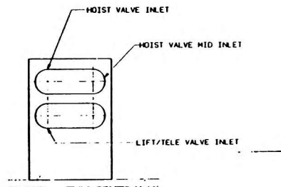
VIEW E-E
